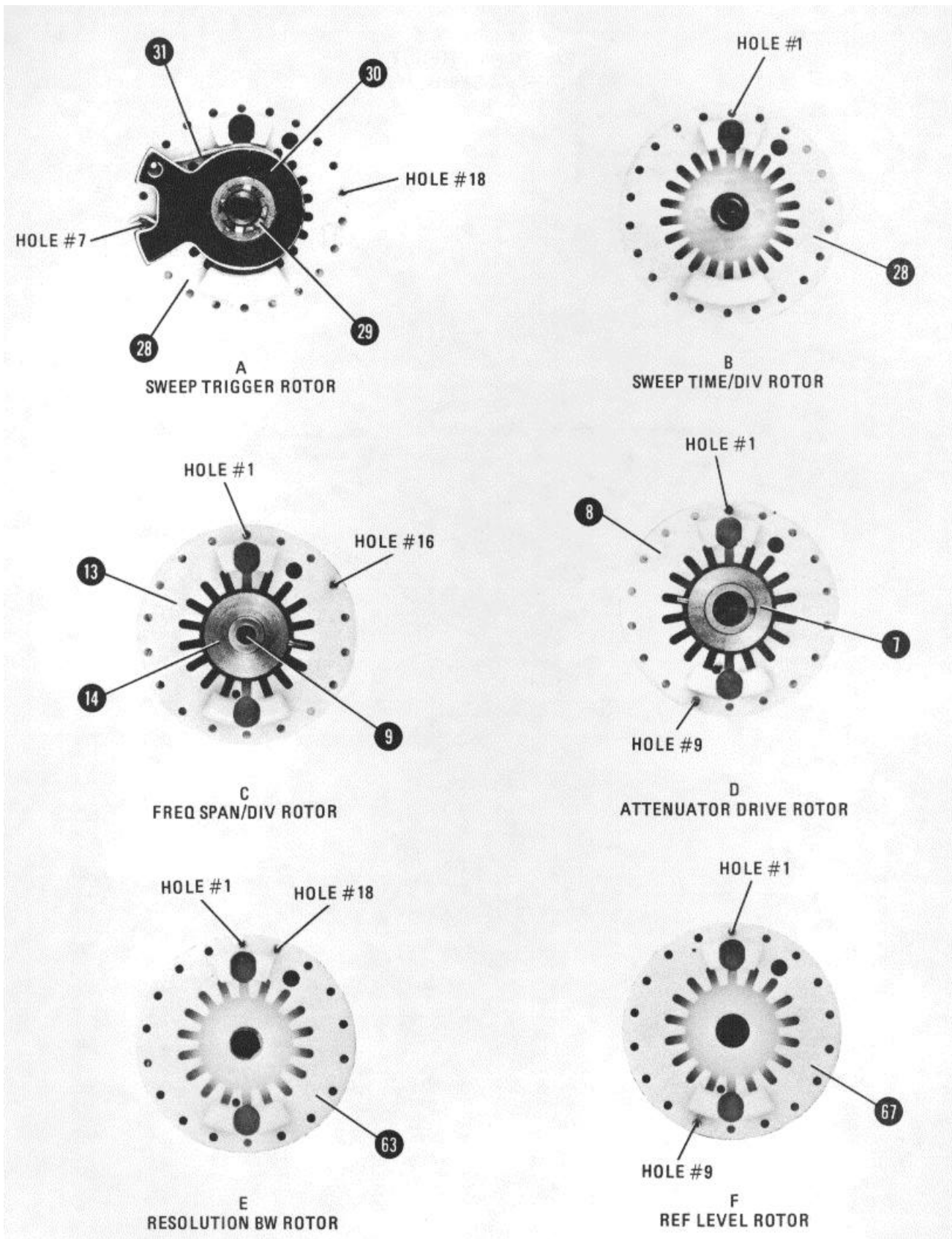
Figure 8-49. Rotor Assemblies
